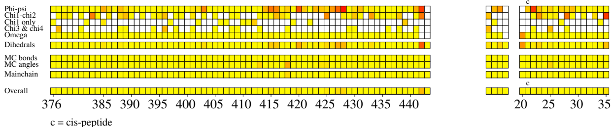
g. G-factors
