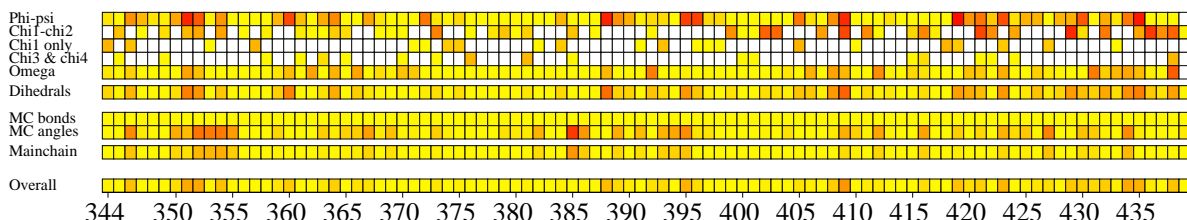
g. G-factors
